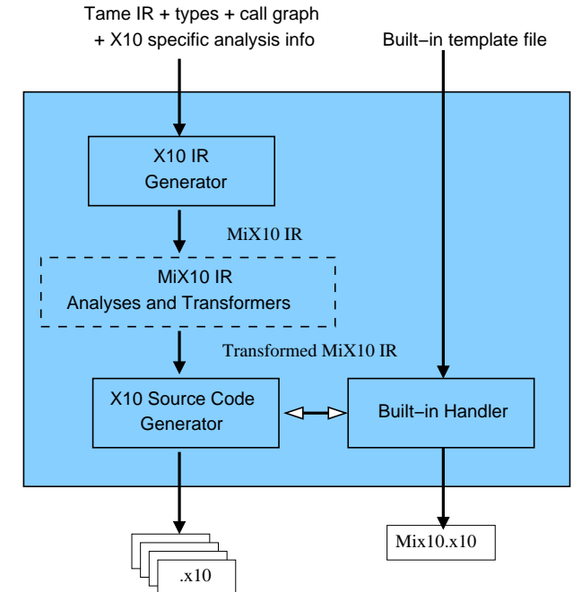
Figure 2. Structure of the MiX10 code generator
