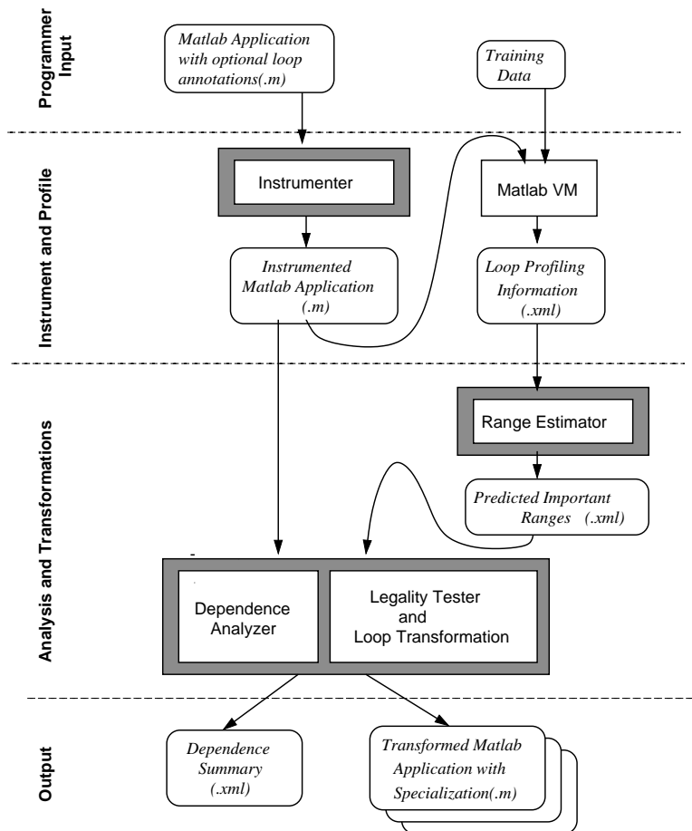
Figure 1: Structure of the McFLAT Framework.
