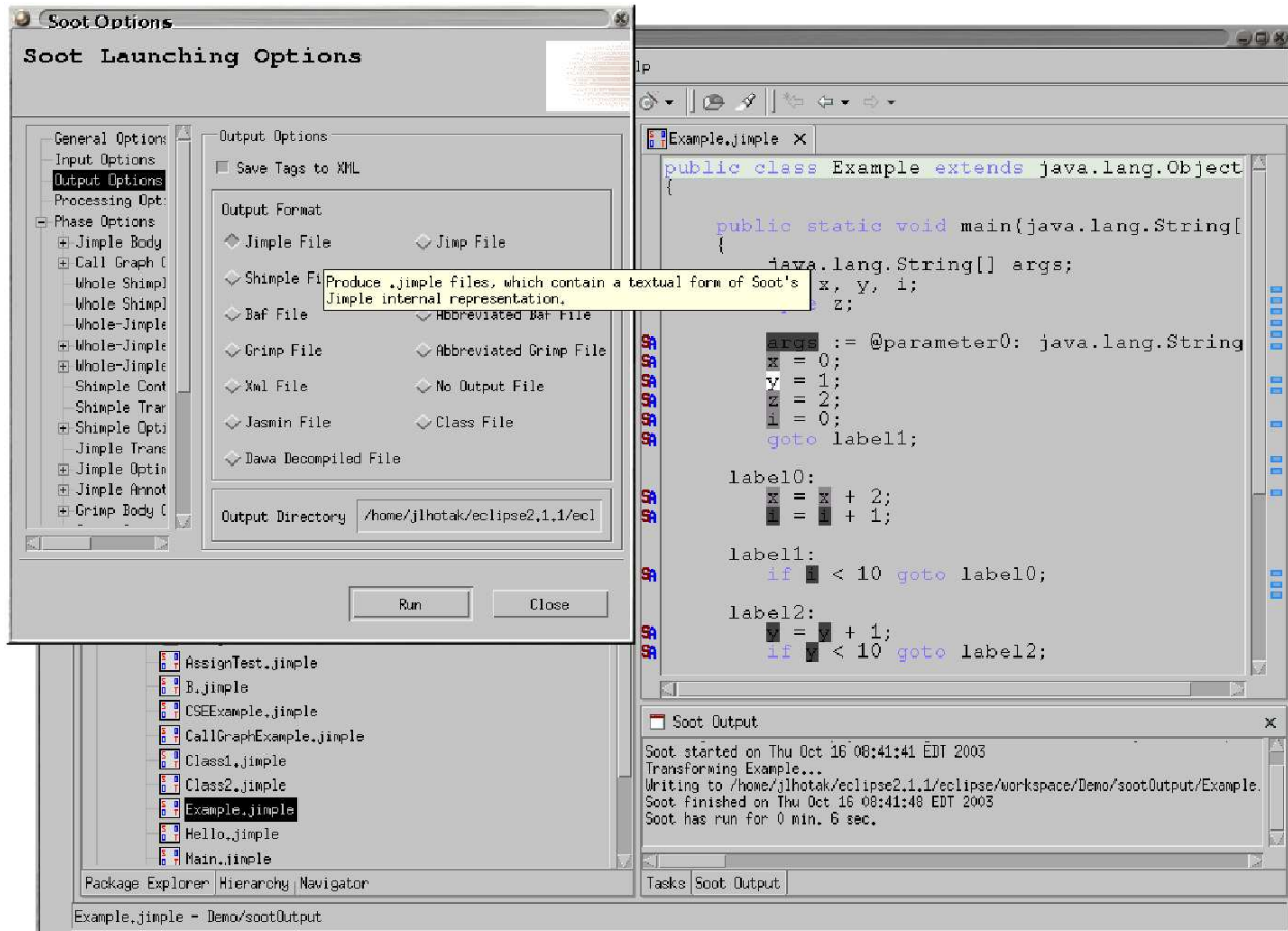
Figure 3: Soot-Eclipse Screenshot
