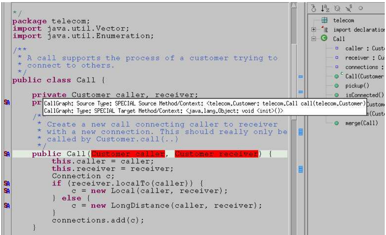
(a) aliased parameters and call graph links
