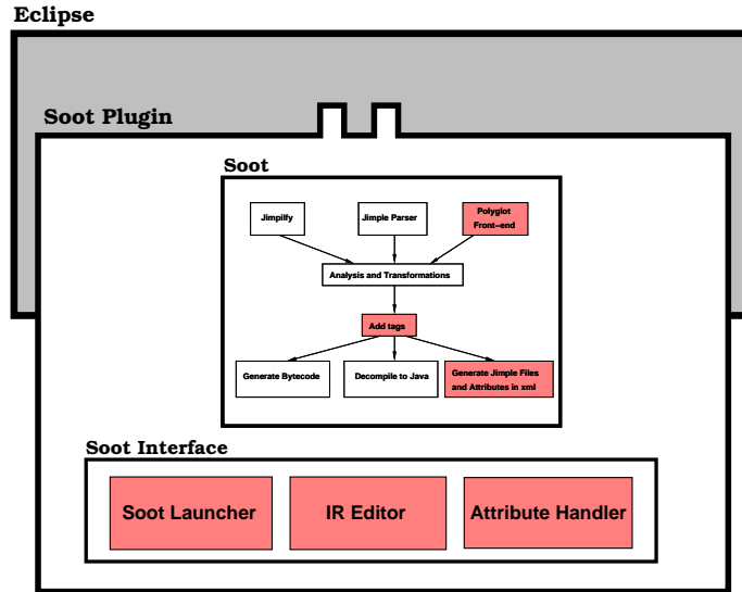
Figure 2: Soot as an Eclipse Plugin
