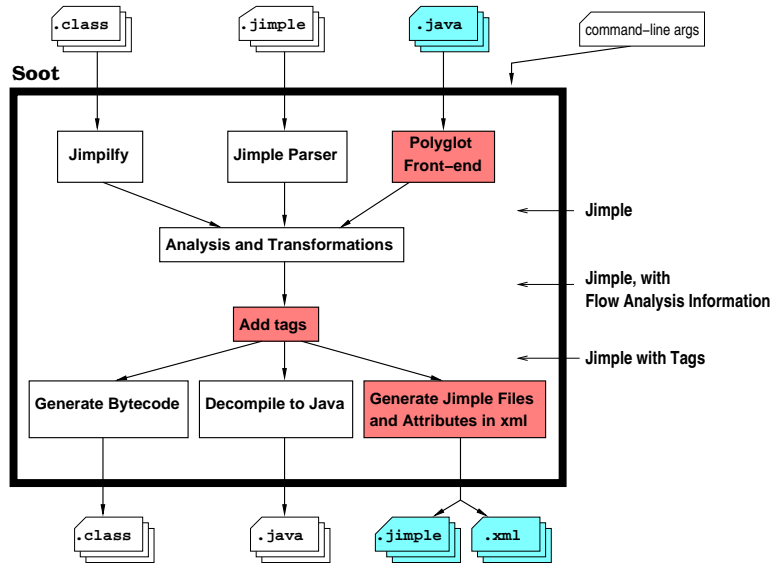
Figure 1: Overview of Soot
