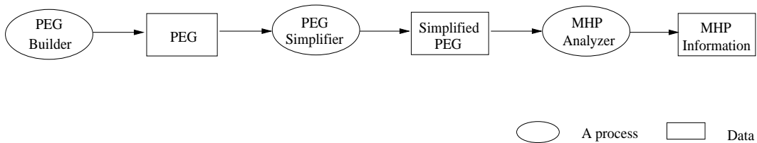
Figure 2: MHP Analysis in Soot.
