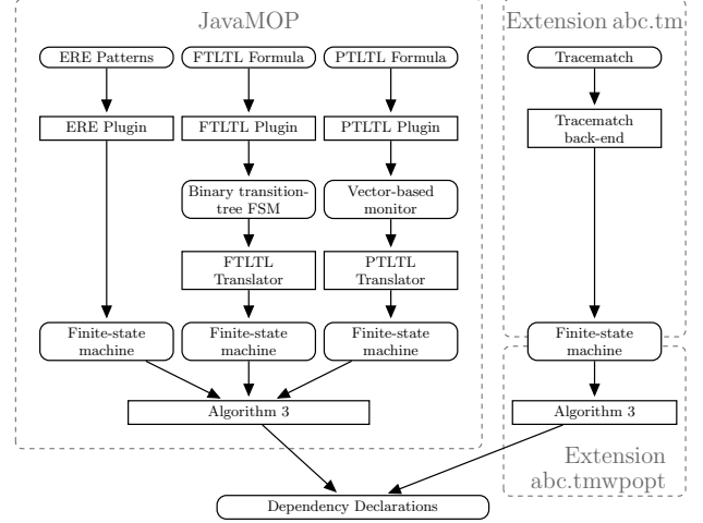
Figure 5: Generating dependent advice in JavaMOP and abc
