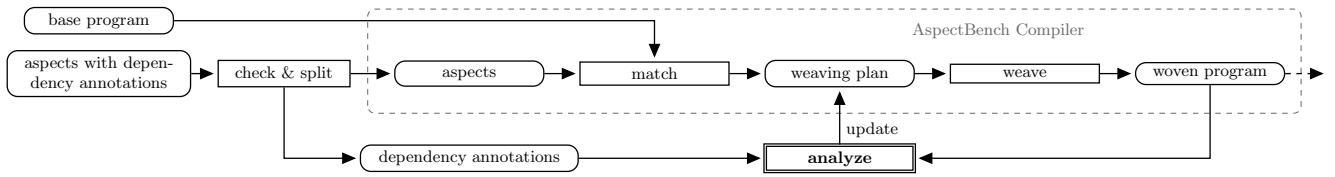
Figure 3: Overview of our implementation of dependent advice as an extension “abc.da” to abc
