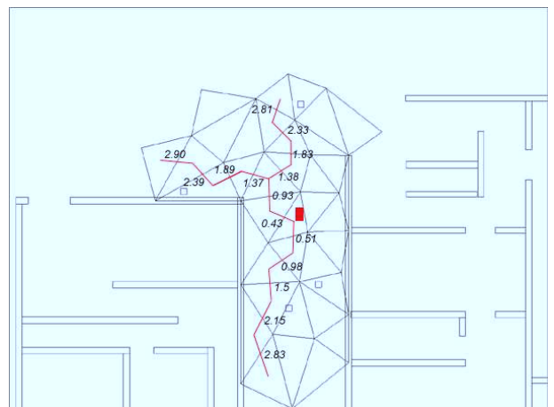
Figure 10: Path distance algorithm with a path length \leq 3.0 . The numbers indicate the path length from the player's tile.
