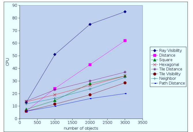
Figure 16: CPU consumption with an increasing number of objects in the world.
