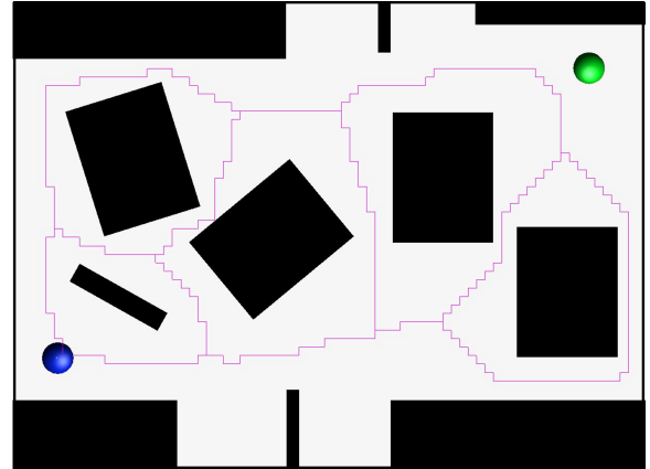
Figure 2: Test level with initial skeleton roadmap. The blue sphere (lower-left) indicates the player start position, and the green sphere (upper-right) the goal.
